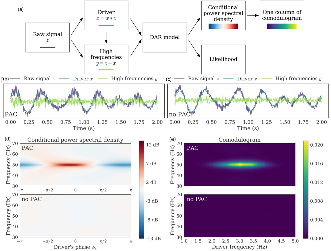
Figure 3.2 – Pipeline, signals, conditional PSD, and comodulograms. (a) Pipeline of the method. We applied it with (p, m) = (10, 1) on two simulated signals: (b) Simulated signal with PAC and (c) Simulated signal without PAC. (d) From a fitted model, we computed the PSD conditionally to the driver’s phase \phi_x ; each line is centered independently to show amplitude modulation. PAC can be identified in the fluctuation of the PSD as the driver’s phase varies: around 50 Hz, the PSD has more power for one phase than for another. This figure corresponds to a single driver’s frequency f_x = 3.0 Hz. (e) Applying this method to a range of driver’s frequency, we build a comodulogram, which quantifies the PAC between each pair of frequencies.
