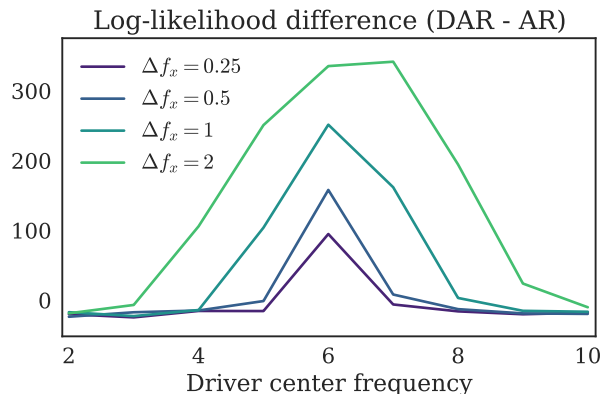
Figure 4.8 – Log-likelihood difference J over a grid of parameters f_x and \Delta f_x , computed on left-out data using cross-validation.
